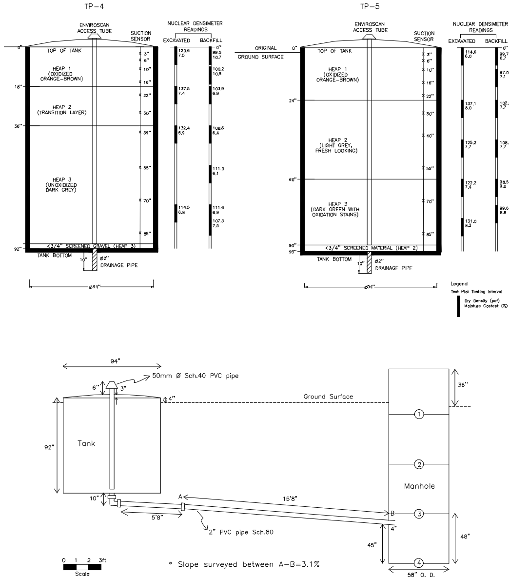
Figure 5. As-built drawings for test plot lysimeters TP-4 and TP-5. The lower panel shows the drain discharge system (for TP-4).
