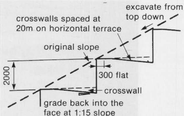
Fig. 7—Design section for terraced slope shown in Fig. 8
