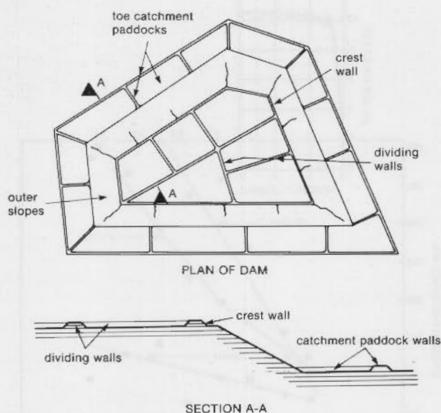
Fig. 2—Diagram showing measures taken to minimize water erosion of abandoned tailings dams
