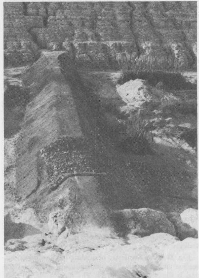
Fig. 11—Appearance of a filter dam with an emergency spillway
