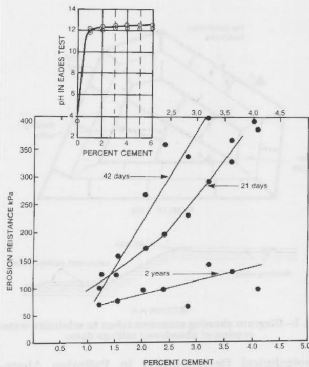
Fig. 4—Results of tests on the stabilization of gold residue with Portland cement
