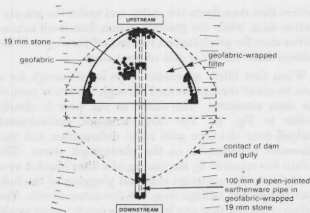
Fig. 10—Plan showing details of a filter dam
