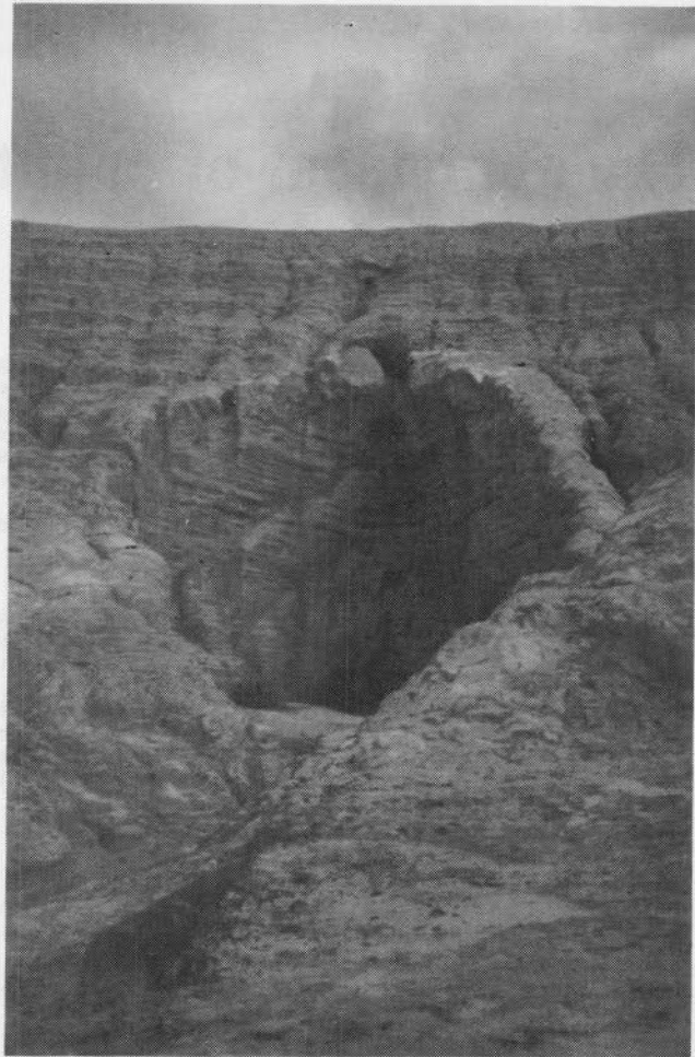
Fig. 1—Severe erosion caused by the collapse of steel penstock and delivery pipes buried in the residue. Voids left by a number of such pipes are visible
